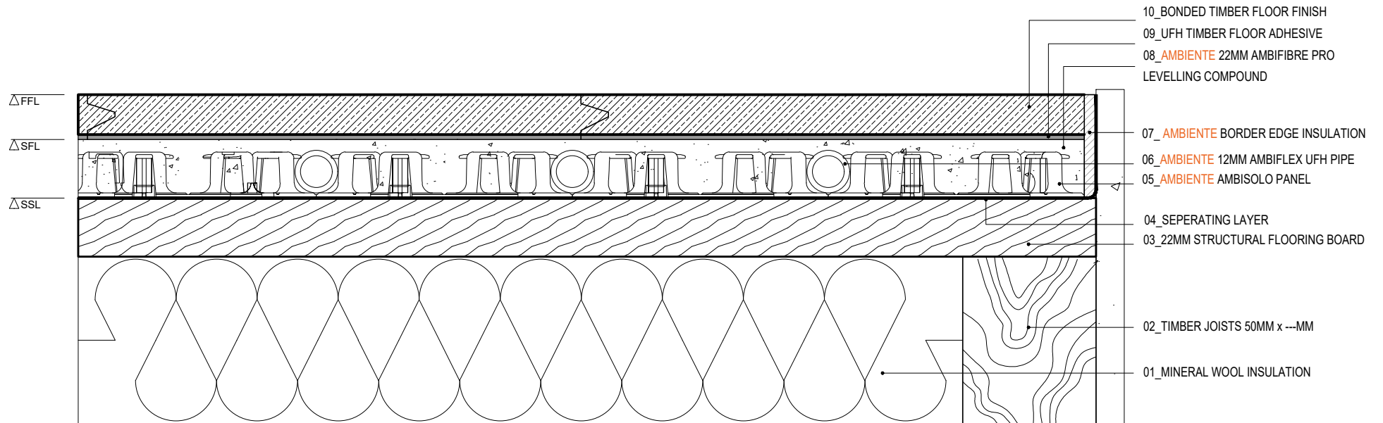
AMBIENTE AMBISOLO SECTION. Bonded Timber Floor Finish - Timber Subfloor
