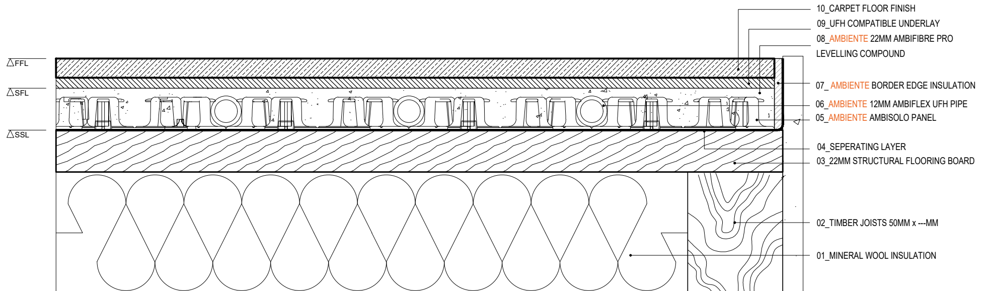
AMBIENTE AMBISOLO SECTION. Carpet Floor Finish - Timber Subfloor
