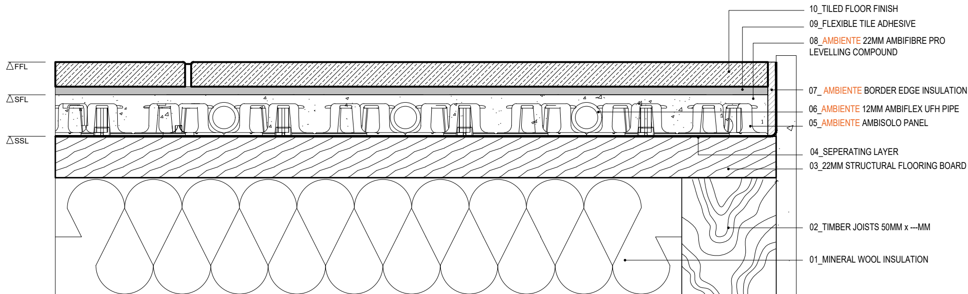
AMBIENTE AMBISOLO SECTION. Tiled Floor Finish - Timber Subfloor
