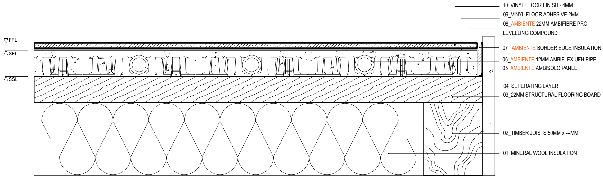
AMBIENTE AMBISOLO SECTION. Vinyl Floor Finish - Timber Subfloor
