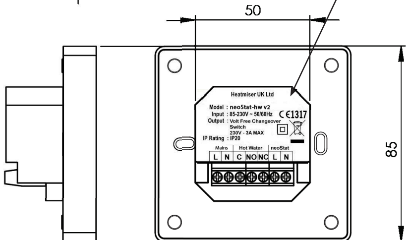
Wiring Detail
