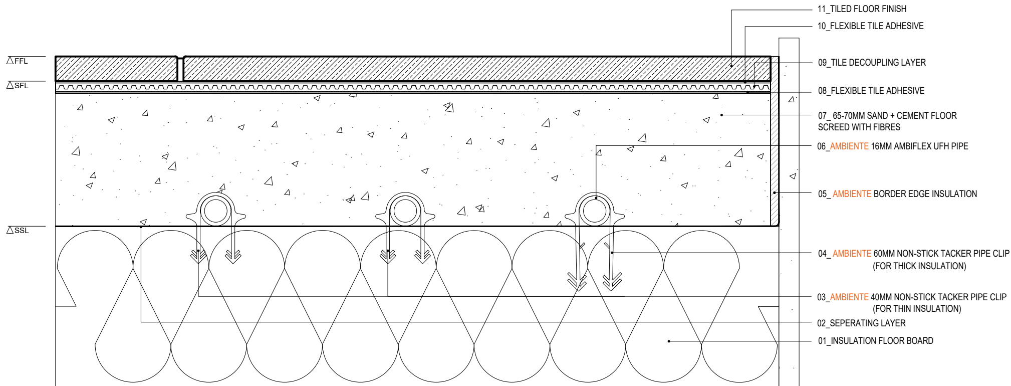
AMBIENTE AMBITAK SECTION. Tiled Floor Finish
