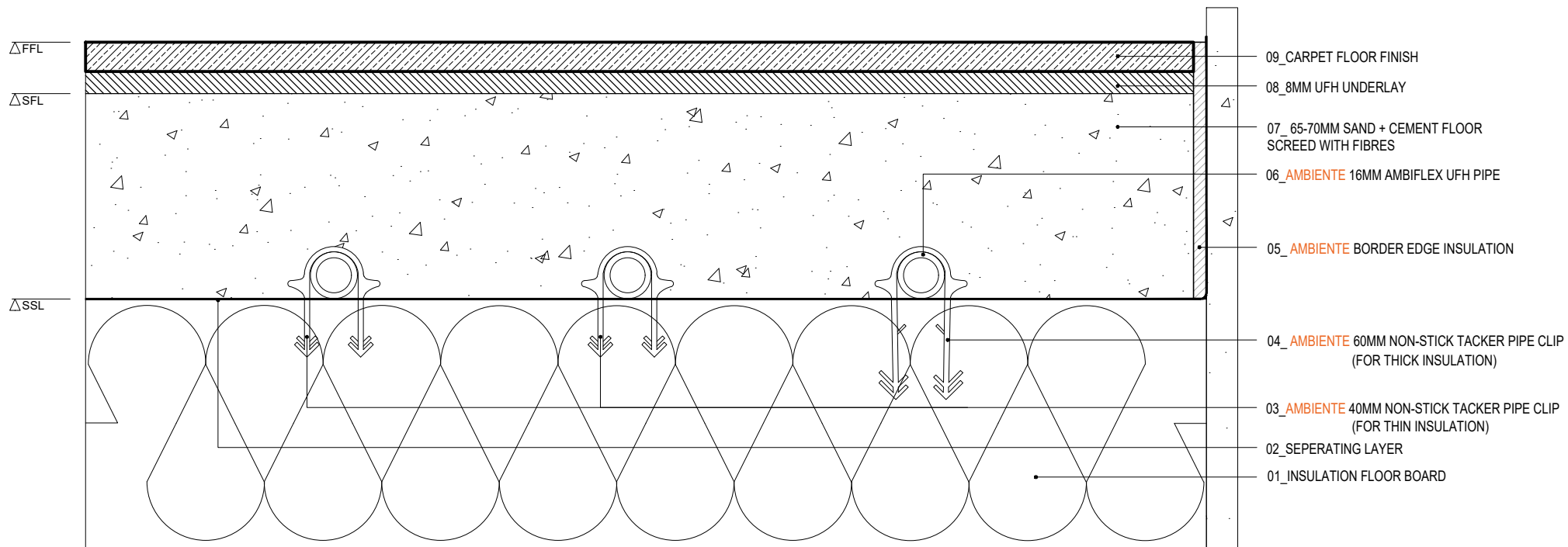
AMBIENTE AMBITAK SECTION. Carpet Floor Finish
