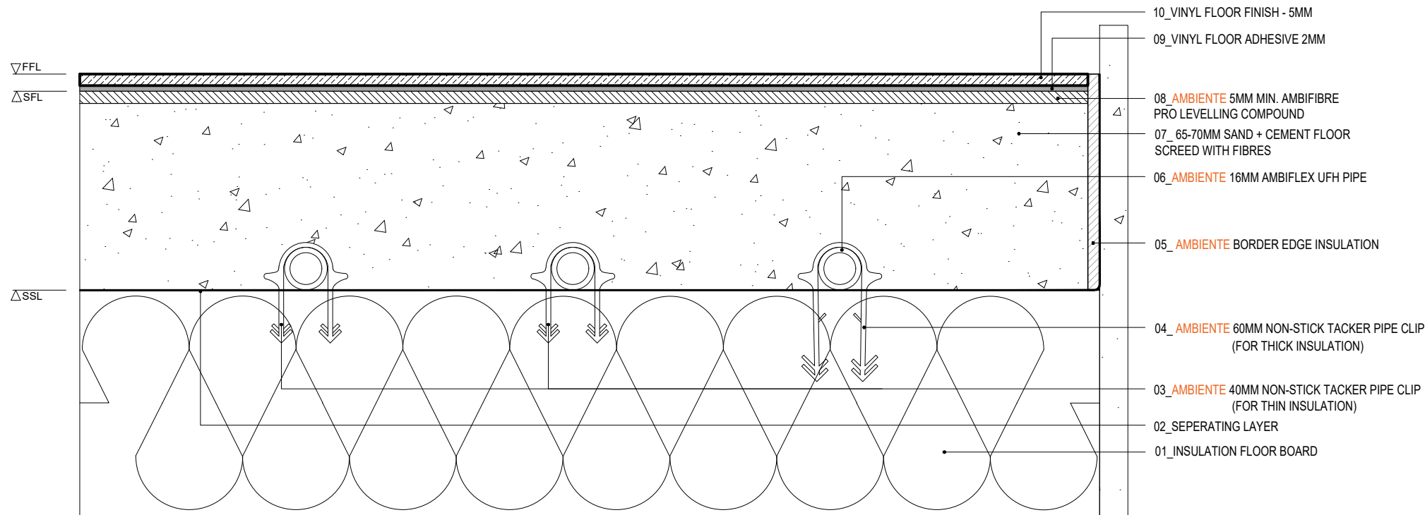
AMBIENTE AMBITAK SECTION. Vinyl Floor Finish
