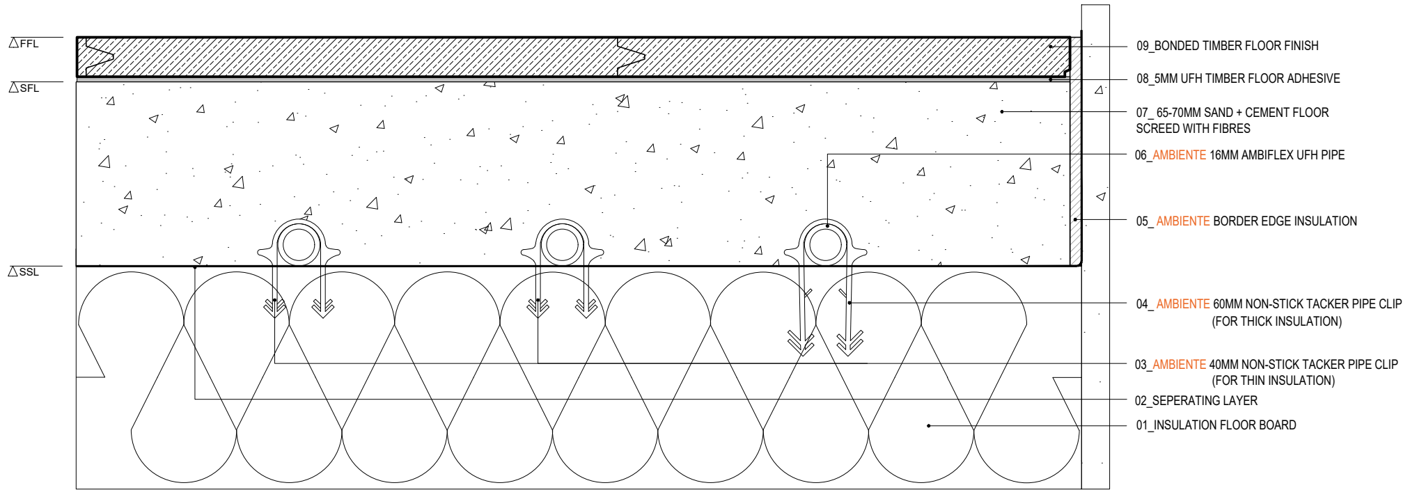
AMBIENTE AMBITAK SECTION. Bonded Wood Floor Finish
