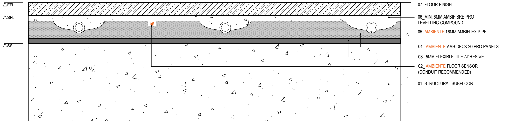
AMBIENTE AMBIDECK 20 PRO. Standard detail - Solid Subfloor
