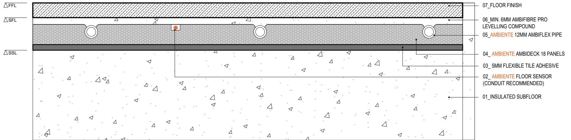
AMBIENTE AMBIDECK 18. Standard detail - Solid Subfloor
