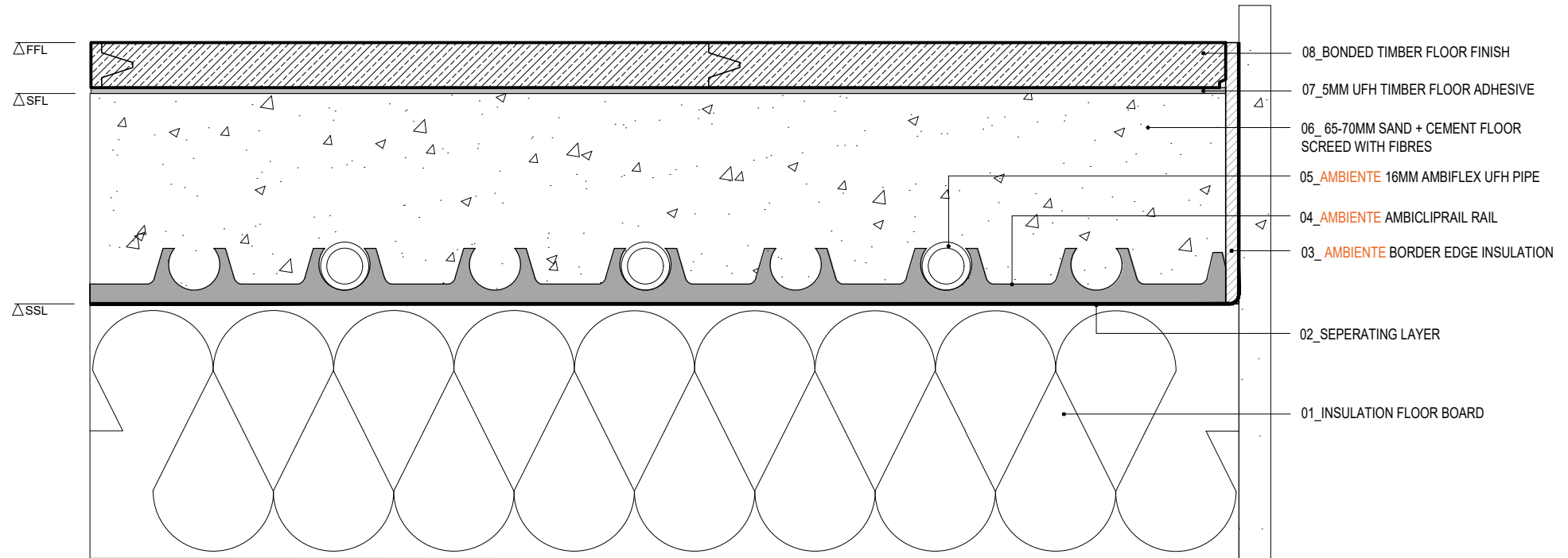
AMBIENTE AMBICLIP SECTION. Bonded Wood Floor Finish
