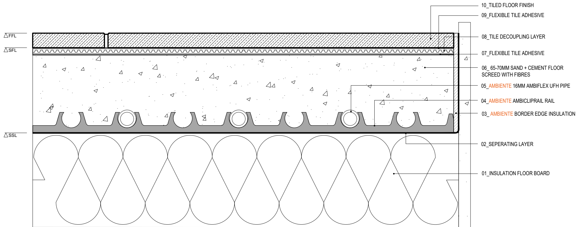
AMBIENTE AMBICLIP SECTION. Tiled Floor Finish
