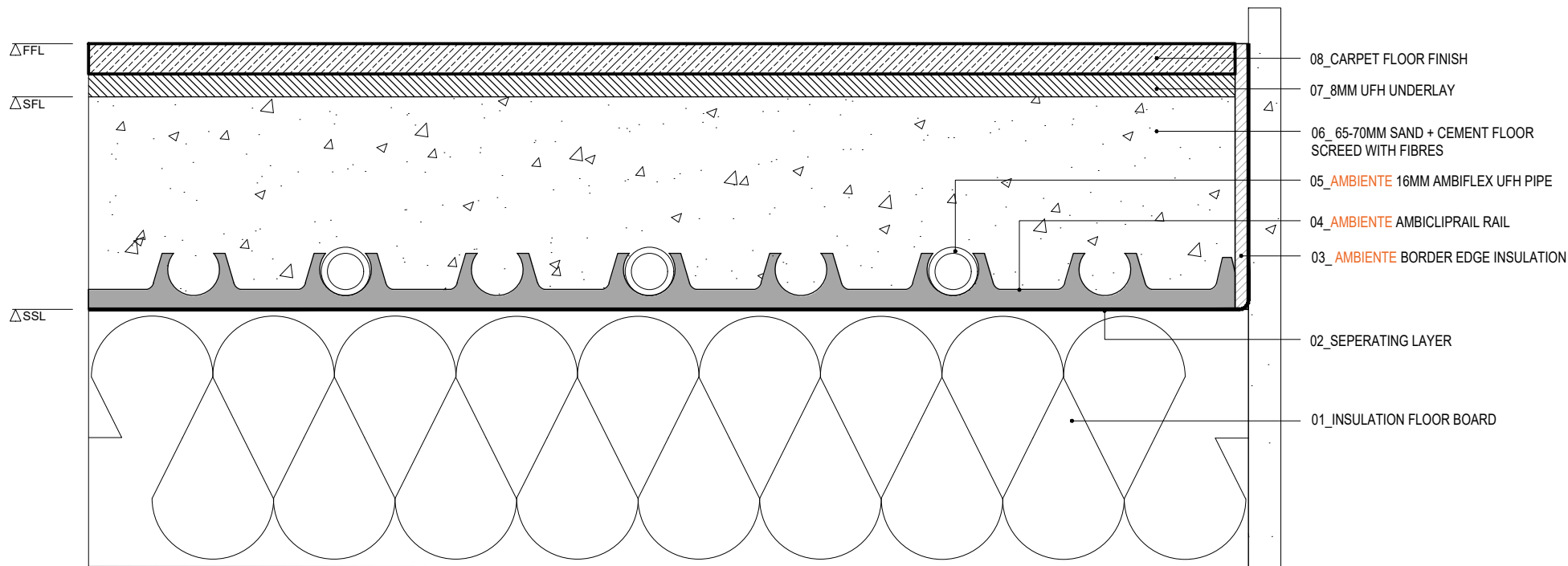
AMBIENTE AMBICLIP SECTION. Carpet Floor Finish
