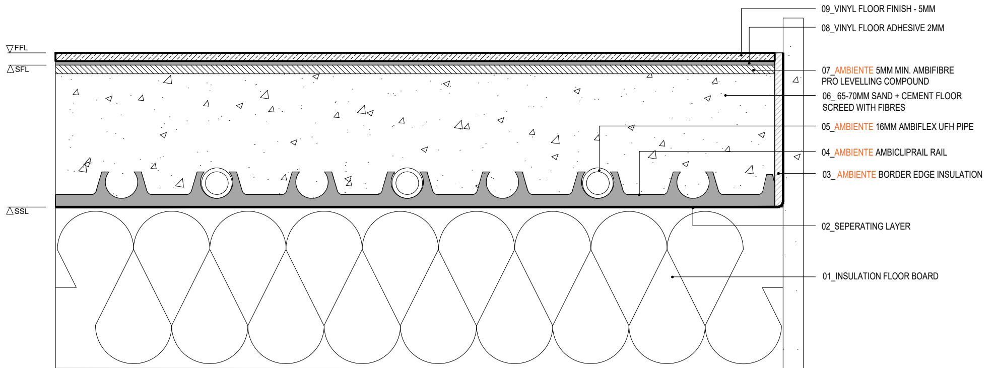
AMBIENTE AMBICLIP SECTION. Vinyl Floor Finish
