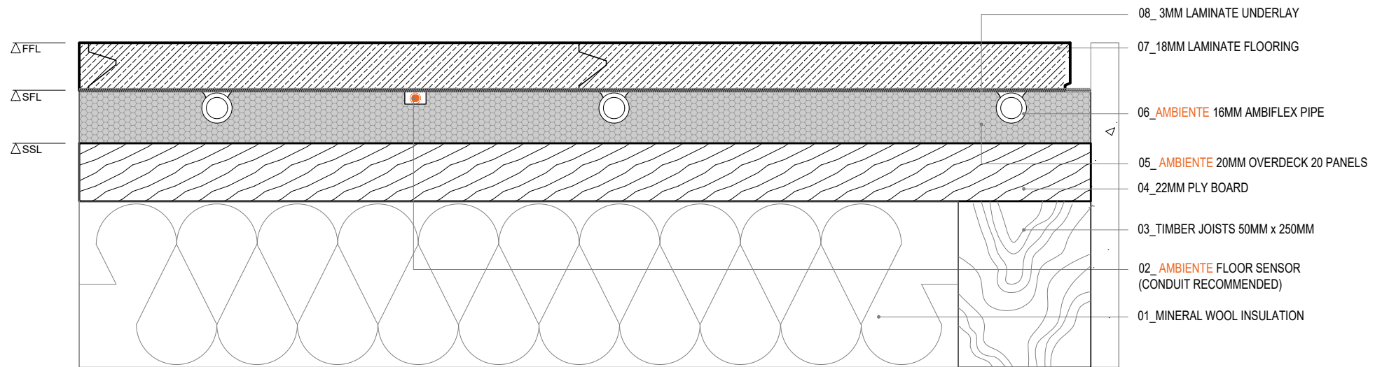
AMBIENTE OVERDECK 20. Laminate Floor Detail - Timber Subfloor
