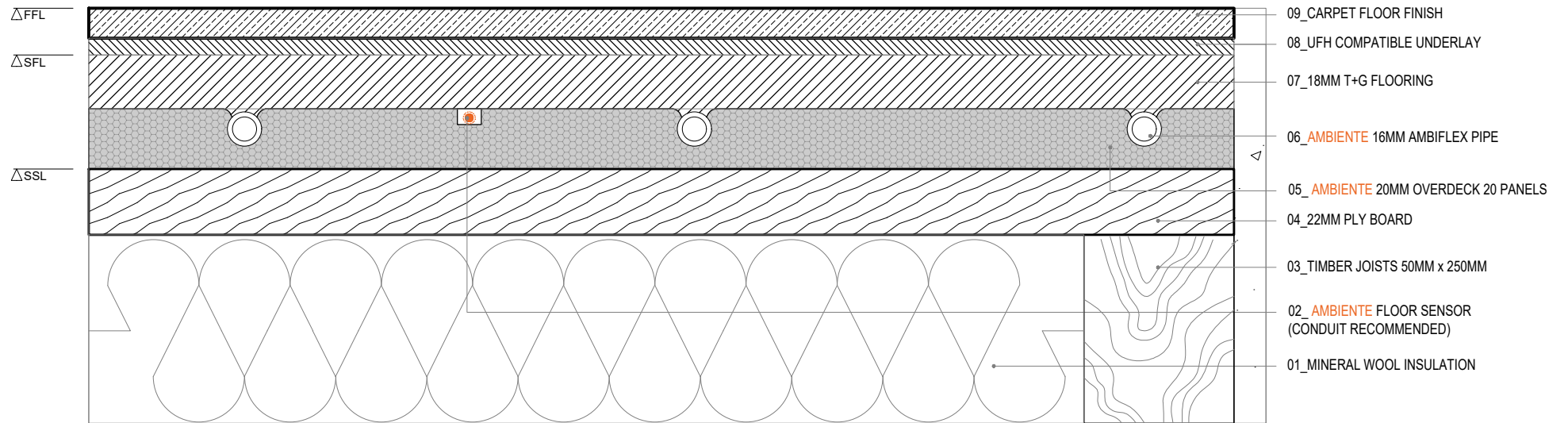
AMBIENTE OVERDECK 20. Carpet Floor Finish - Timber Subfloor
