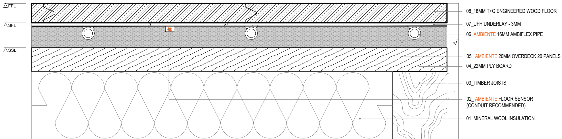
AMBIENTE OVERDECK 20. Wood Floor Detail - Timber Subfloor
