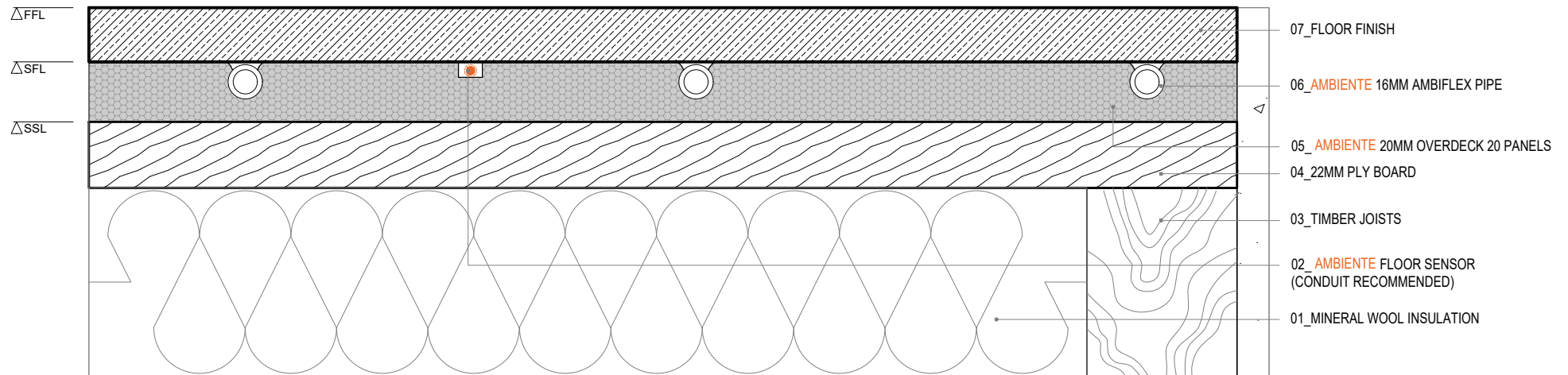
AMBIENTE OVERDECK 20. Standard Floor Detail - Timber Subfloor
