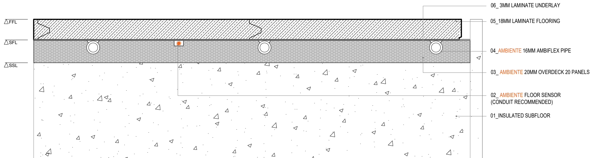
AMBIENTE OVERDECK 20. Laminate Floor Detail - Solid Subfloor
