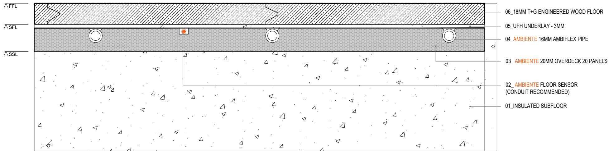
AMBIENTE OVERDECK 20. Wood Floor Detail - Solid Subfloor
