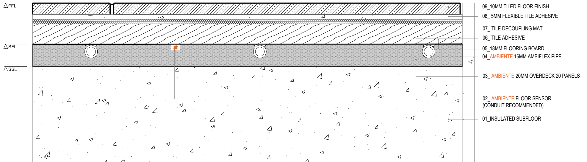
AMBIENTE OVERDECK 20. Tiled Floor Finish - Solid Subfloor
