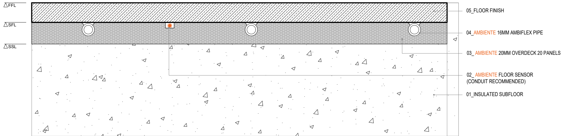
AMBIENTE OVERDECK 20. Standard Floor Detail - Solid Subfloor
