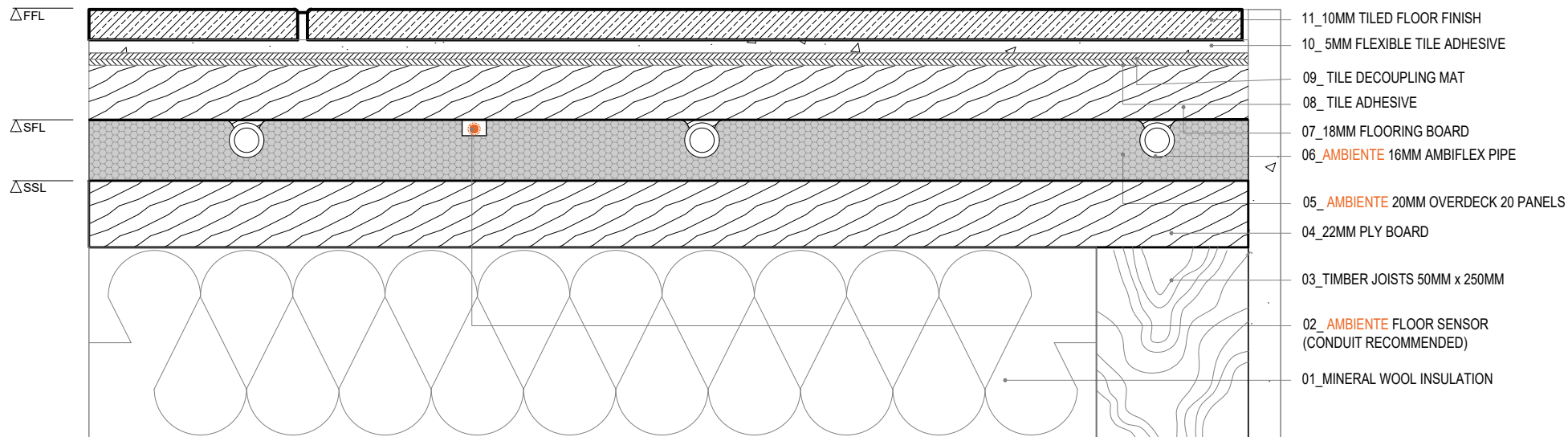
AMBIENTE OVERDECK 20. Tiled Floor Finish - Timber Subfloor
