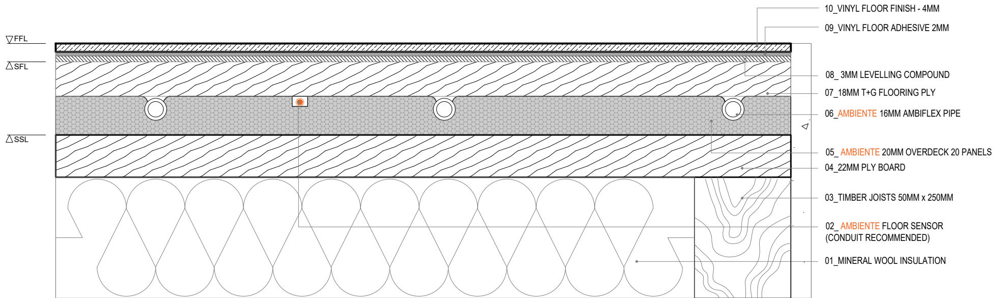
AMBIENTE OVERDECK 20. Vinyl Floor Finish - Timber Subfloor
