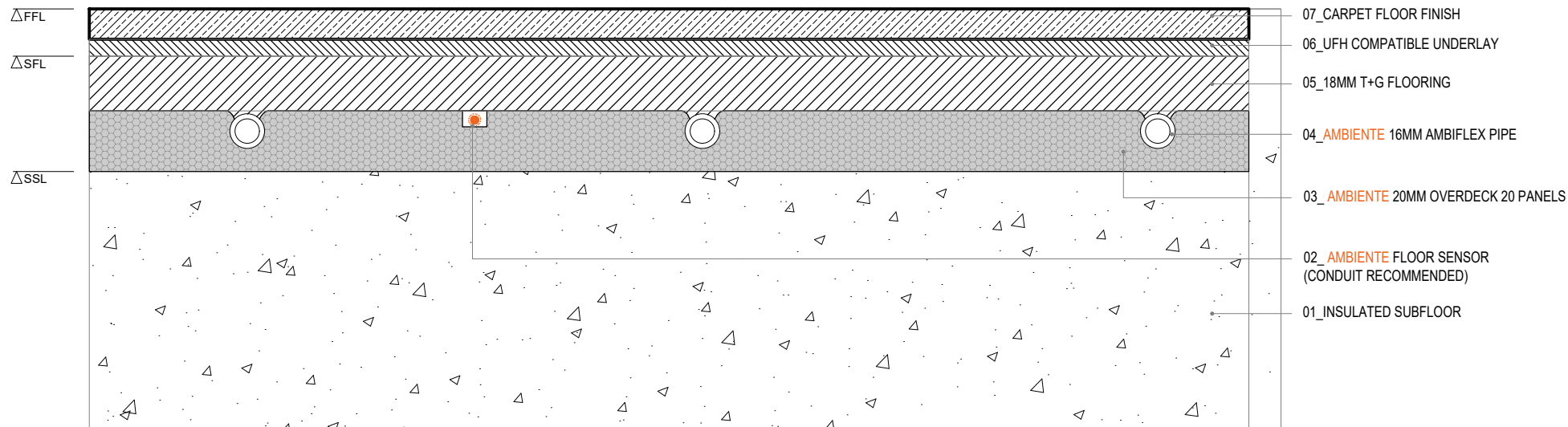
AMBIENTE OVERDECK 20. Carpet Floor Finish - Solid Subfloor
