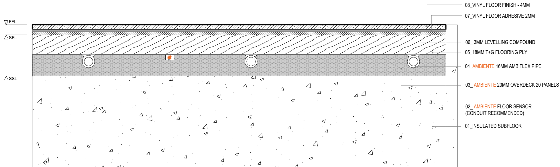
AMBIENTE OVERDECK 20. Vinyl Floor Finish - Solid Subfloor
