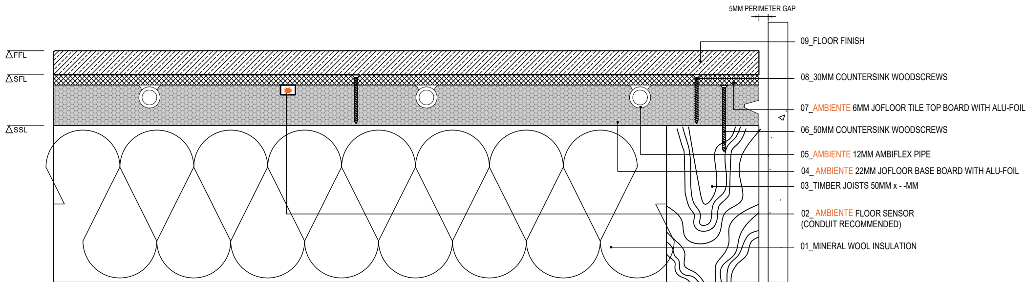
AMBIENTE JOFLOOR 28. Standard Floor Finish
