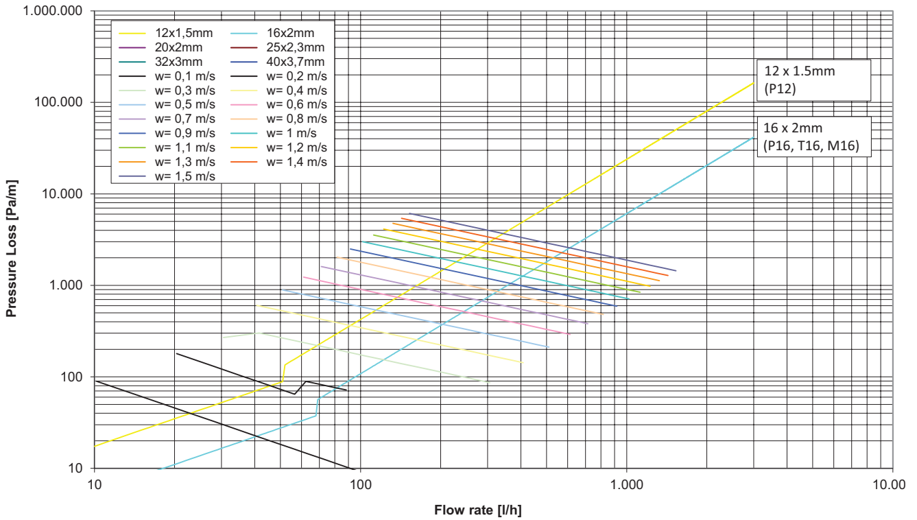
Linear Pressure Loss Diagram for P12, P16, T16 & M16 PERT pipes
